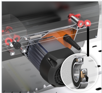
CARRIAGE The carriage motor group slides with 8 ball-bearings on an interchangeable stainless steel track.
