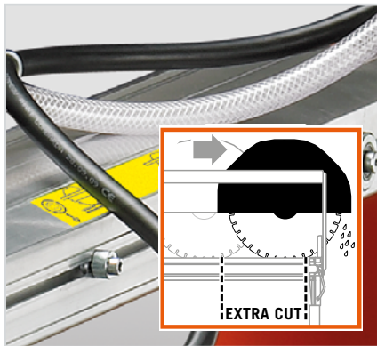
EXTRA CUT Adjusting the end-run-carriage, it increases the cutting length.
